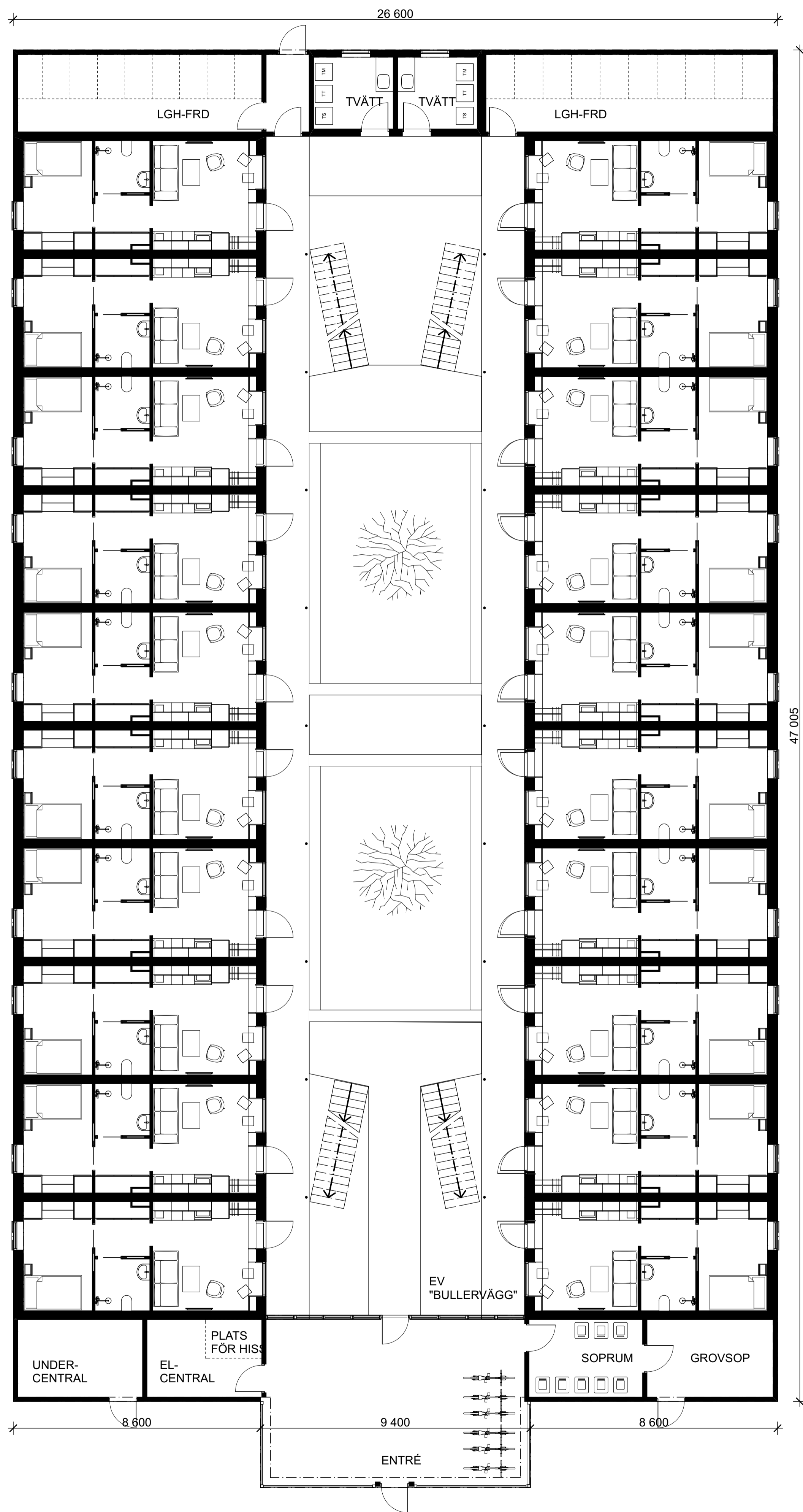
Story 1:100
