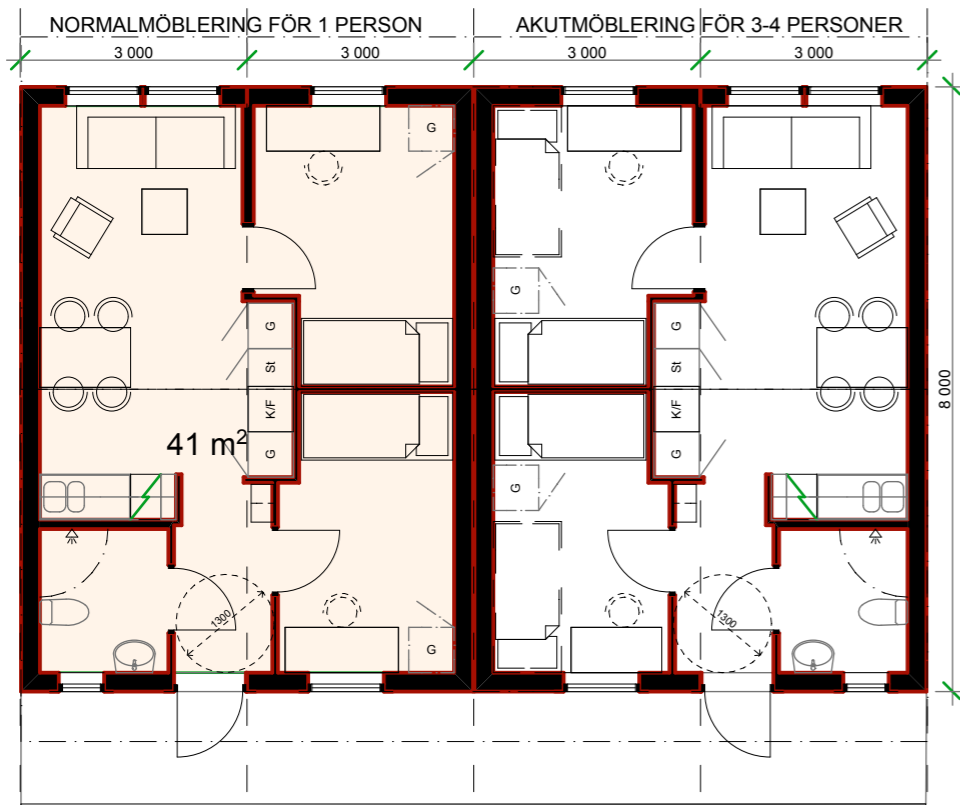
2. Story 1:100
