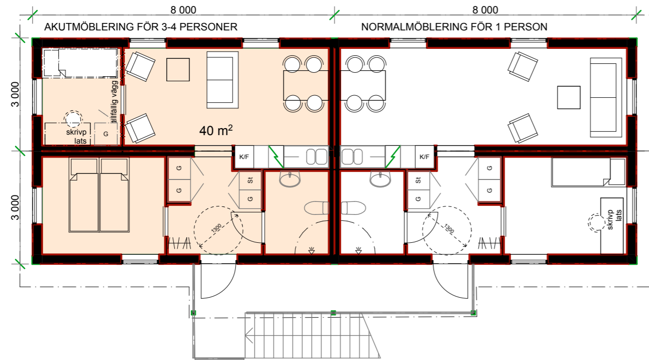
2. Story 1:100
