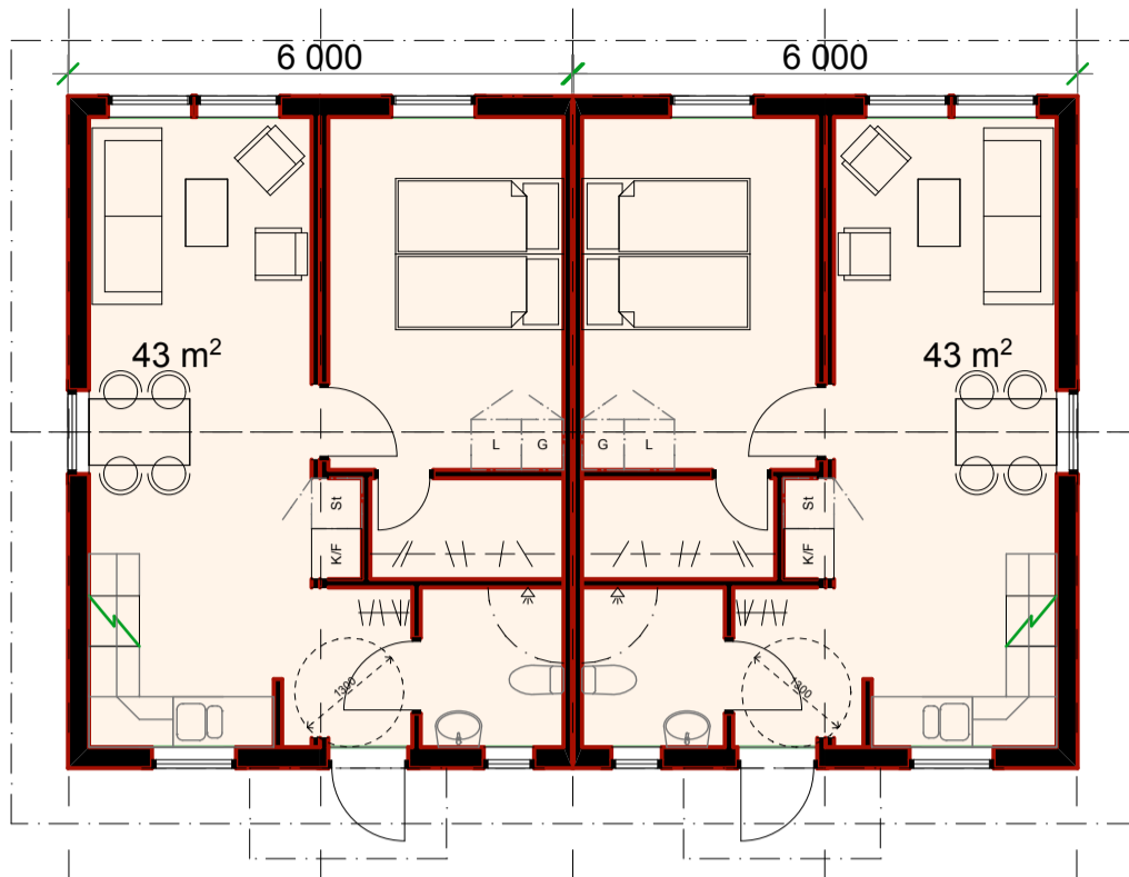
0. Story (3) 1:100
