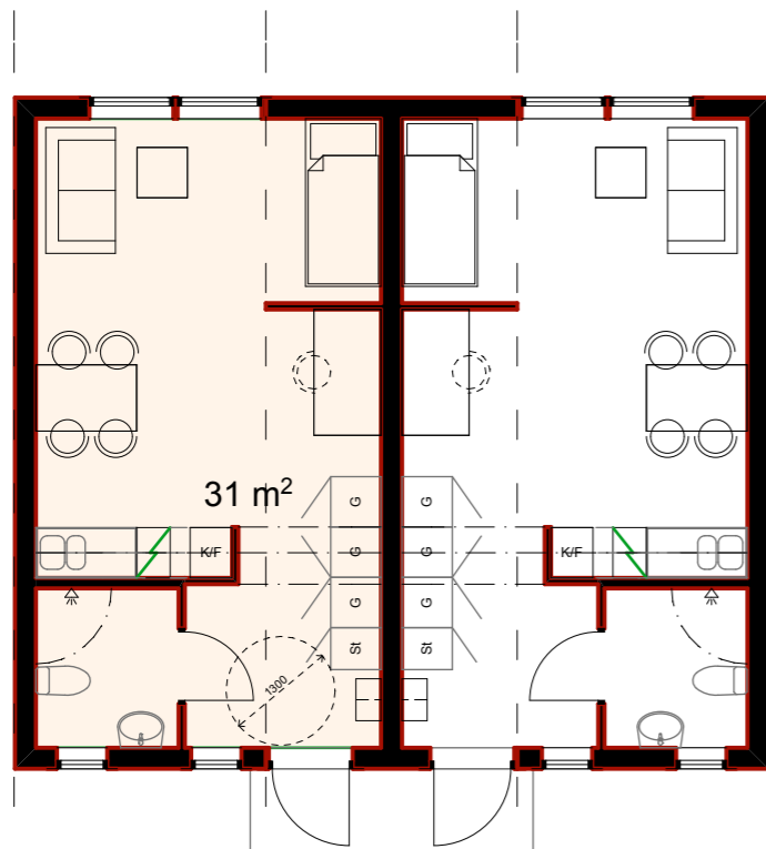
1. Story 1:100
