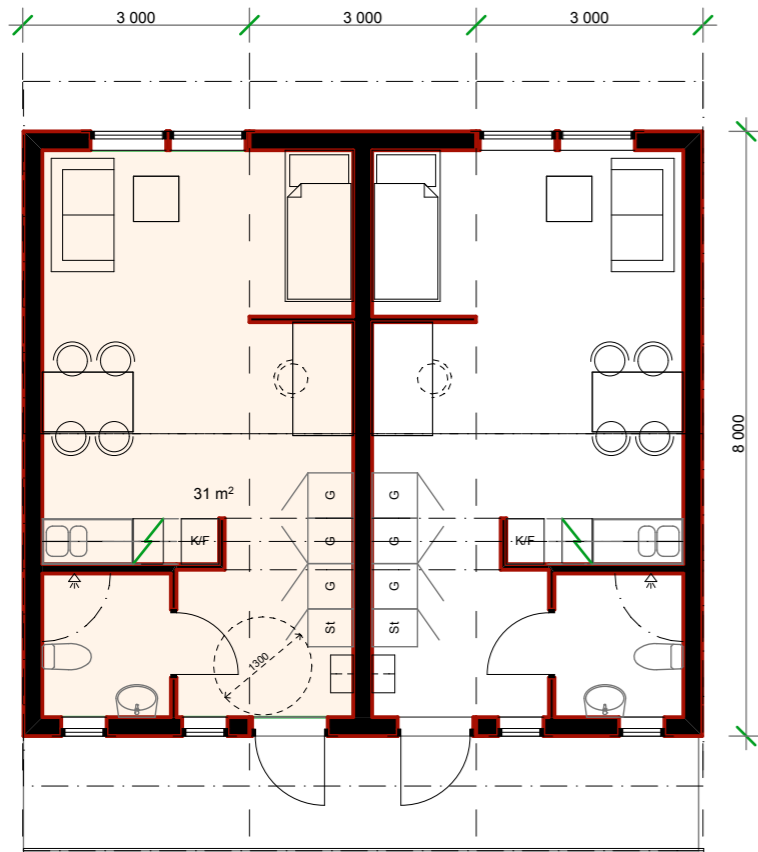
2. Story 1:100
