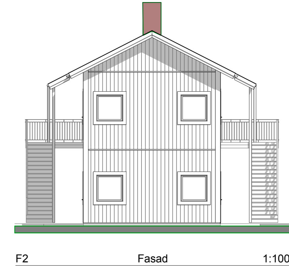
1. Story 1:100
